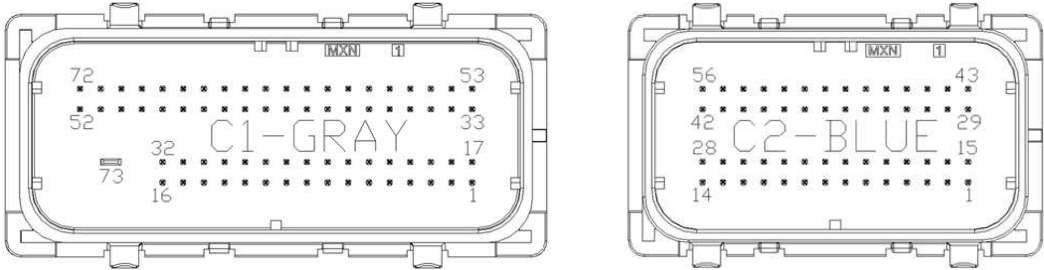
AEM Infinity Connectors Viewed from Wire Side
