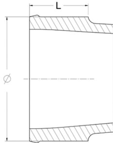
Compressor Outlet HOSE CONNECTIONS ∅ 63.5 X 30
