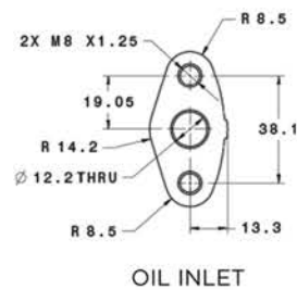
OIL INLET
