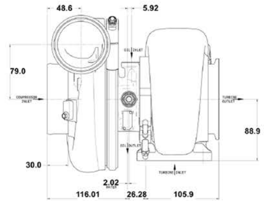
G42-1200 Compact
