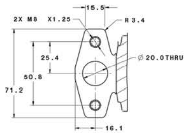
OIL OUTLET
